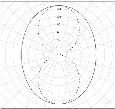
cd/klm — C0 - C180 - - - C90 - C270 η = 100%
